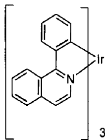
Ir(1-piq) 3
